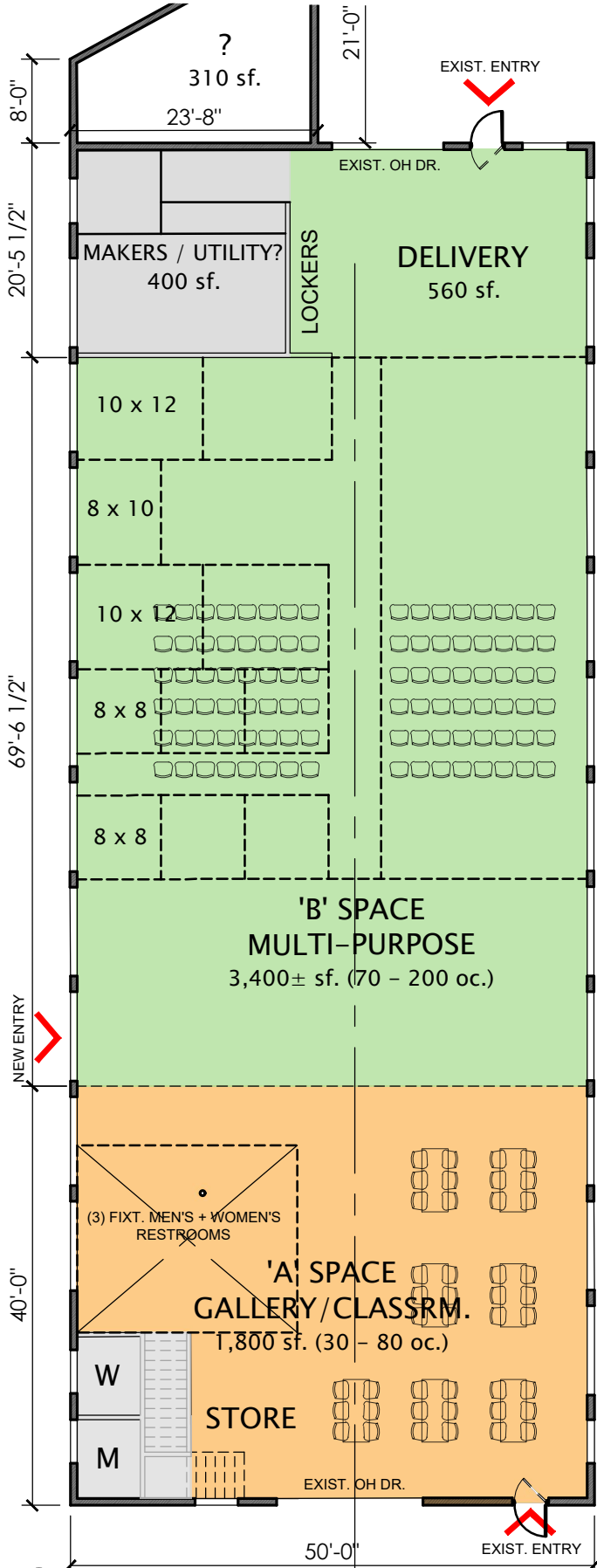
1 1ST FLOOR PLAN A101 1/16" = 1'-0"
