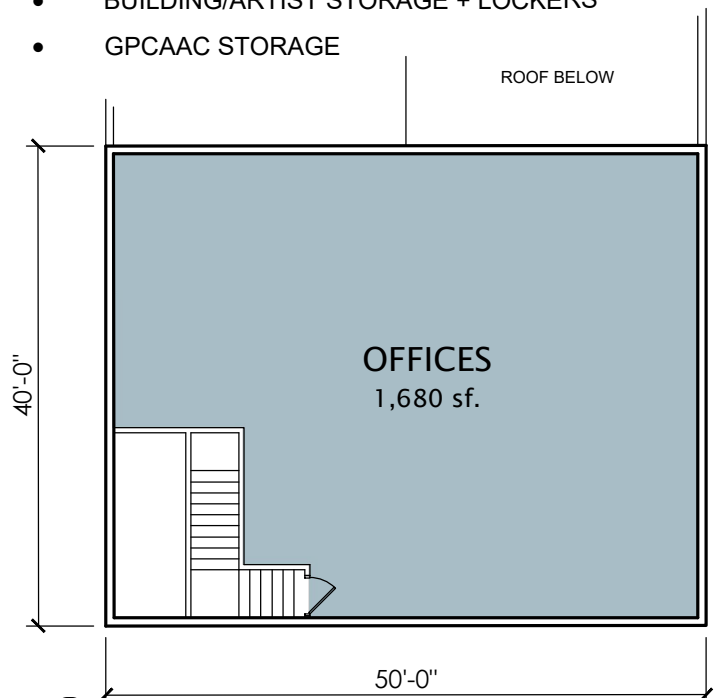
2 2ND FLOOR PLAN A101 1/16" = 1'-0"
